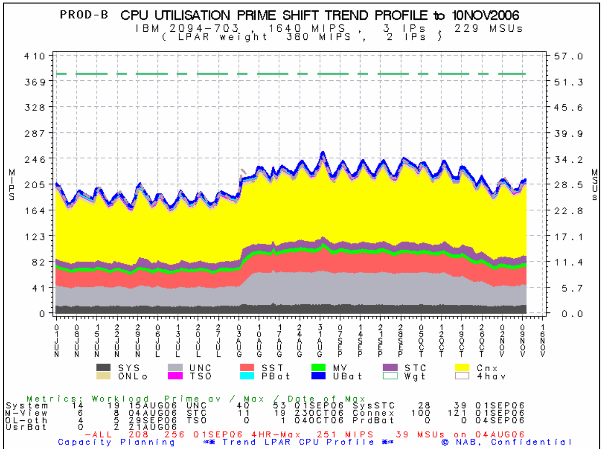
Chart 9: PROD-B LPAR Prime Shift Trends - Workload breakdown
