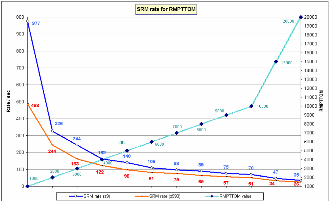
Chart 5: SRM Chart for RMPTTOM setting z9 EC and z990 processors- invocation interval : rate/sec
