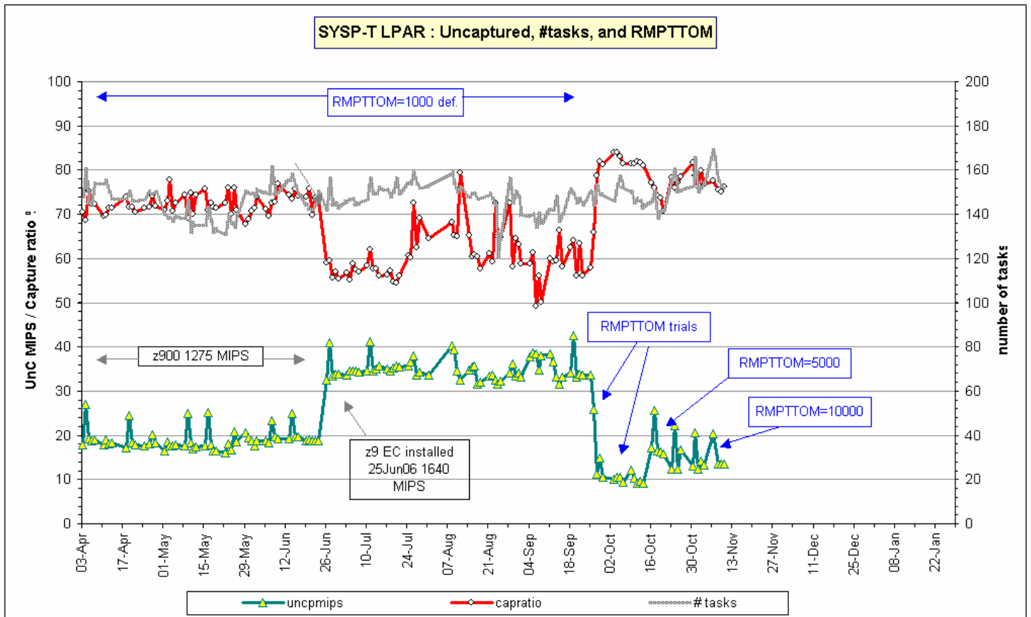
Chart 1: SYSP-T LPAR trends of metrics of interest – Prime Shift Averages
